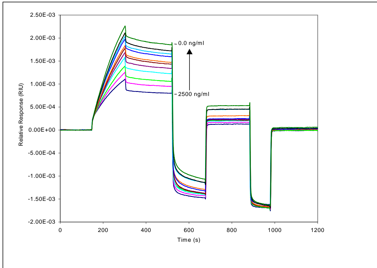
Figure 1. Overlaid sensorgrams for binding of anti-biotin to the BSA-biotin-coated surface. Each sample contains 2500.0, 1250.0, 625.0, 312.5, 156.2, 78.1, 39.0, 19.5, 9.7, 4.9, 2.4 and 0.0 ng/ml of biotin, respectively. The antibody binding response is inversely proportional to the biotin concentration.
